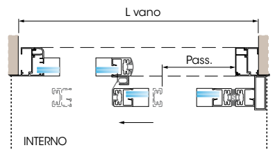
Horizontal section ASD 1+1, profile 32 mm
