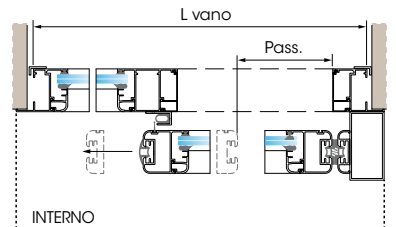
Horizontal section ASD 1+1, profile 50 mm
