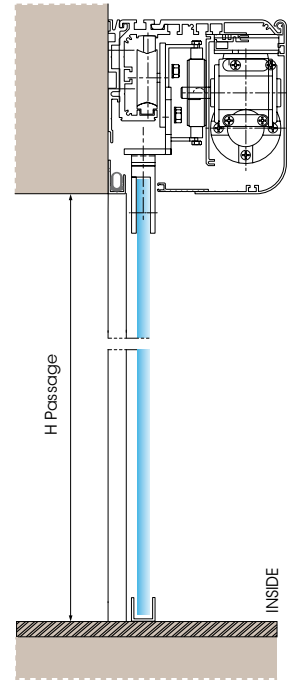
Vertical section GLAZED 2A Solution with glass doors tempered or laminated 10mm
