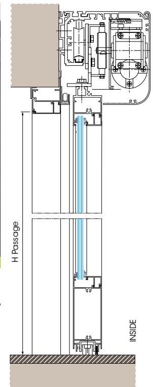
Vertical section ASD2 door Ponzi profile 50 mm series Pvb laminated glass 0.76 mm
