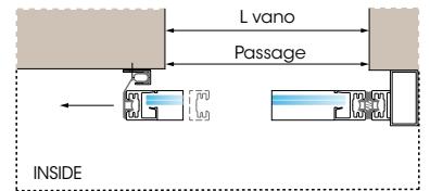
Horizontal section ASD 1, profile 32 mm
