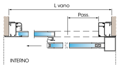
Horizontal section ASD 1+1, profile 20 mm
