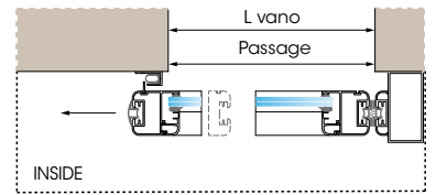
Horizontal section ASD 1, profile 50 mm
