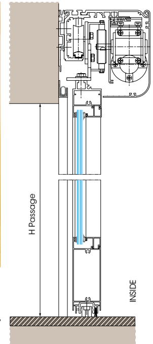
Vertical section ASD2 door Ponzi profile 50 mm series Pvb laminated glass 0.76 mm
