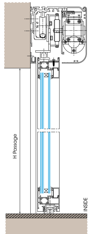
Vertical Section T.T. door Thermal Cut Profile 62 mm Very thick insulating glass
