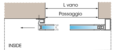
Horizontal section ASD 1, profile 20 mm
